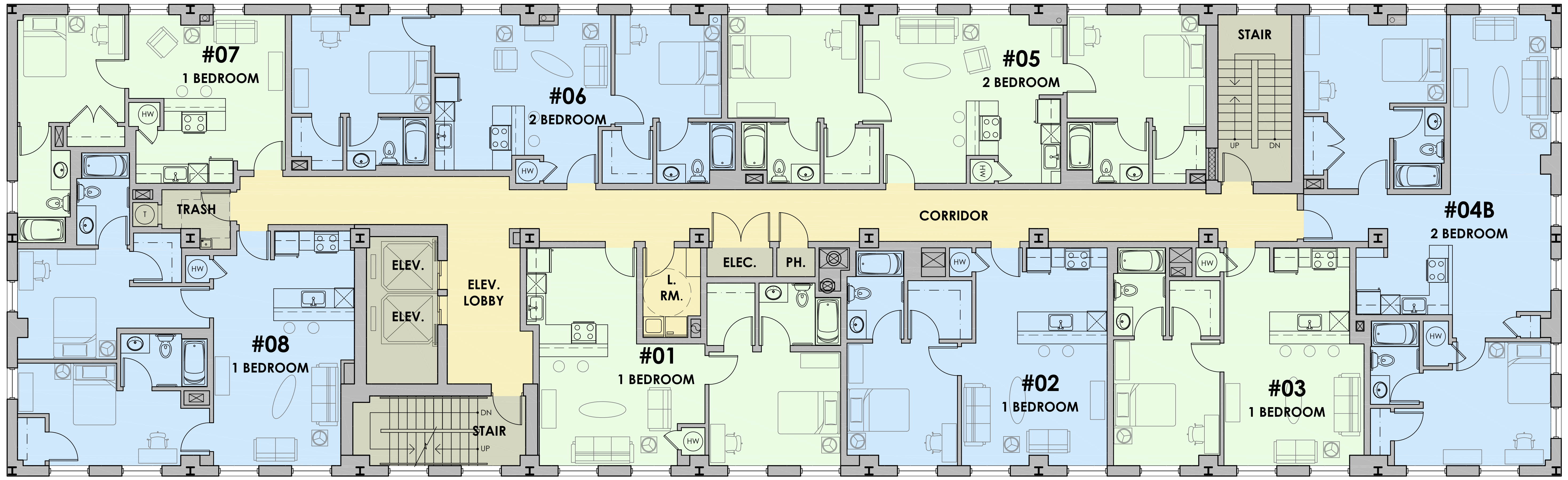
TYPICAL FLOOR PLAN-FLOORS 4 & 5 & 6
